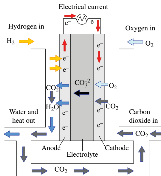
FIGURE 30.16 Molten carbonate fuel cell. Photo courtesy of EERE, Department of Energy.
