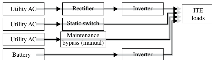
FIGURE 27.11 Multiple power delivery paths to get power to the connected loads. Courtesy of Eaton.
