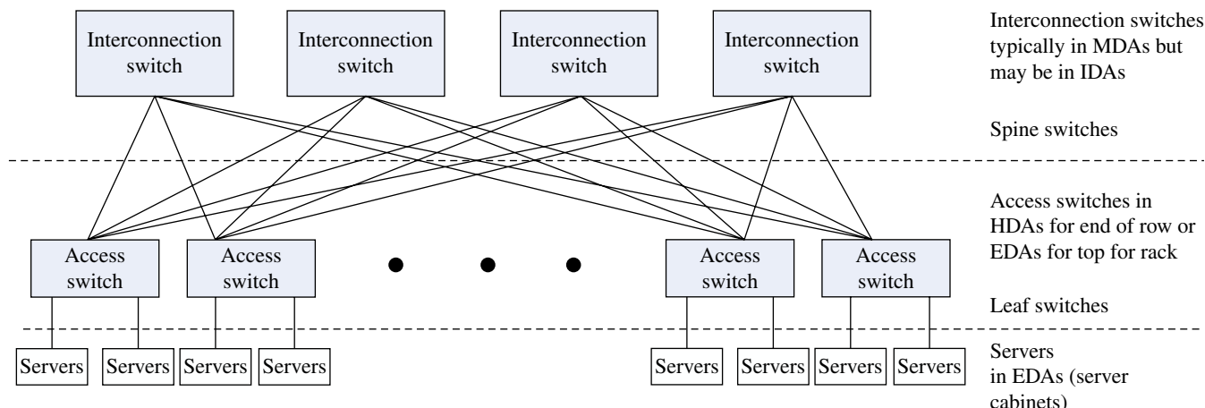
FIGURE 14.12 Data center switch fabric example.
