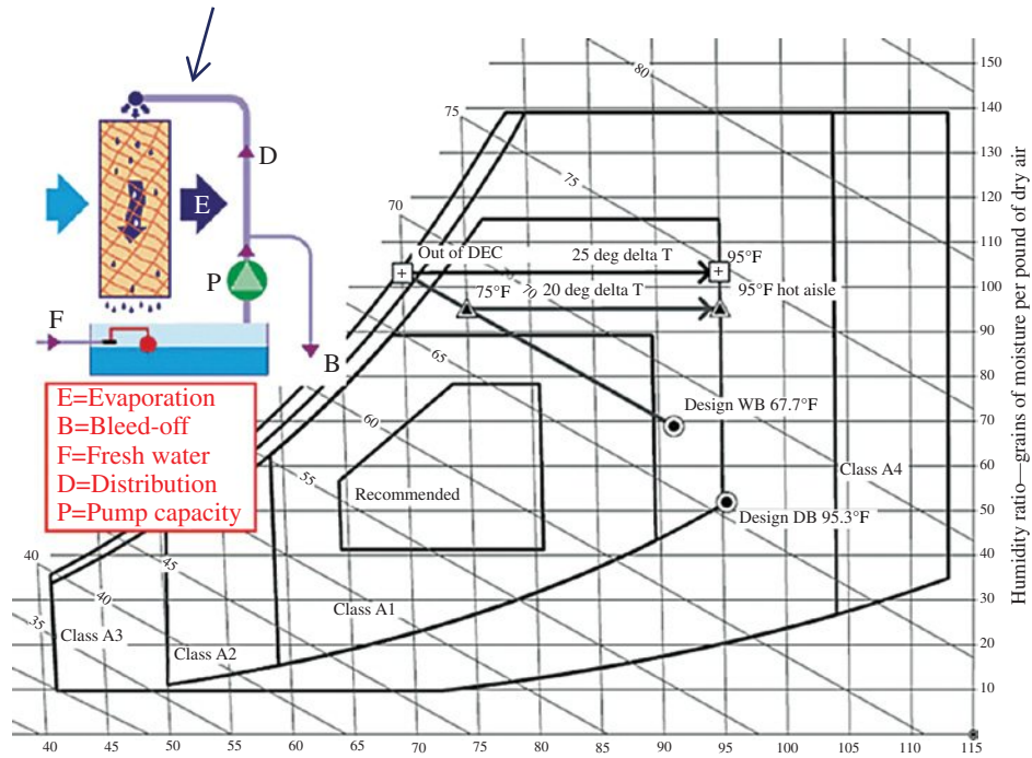
FIGURE 25.2 Direct cooling processes shown with recommended and allowable envelopes for datacom supply temperature and moisture levels.
