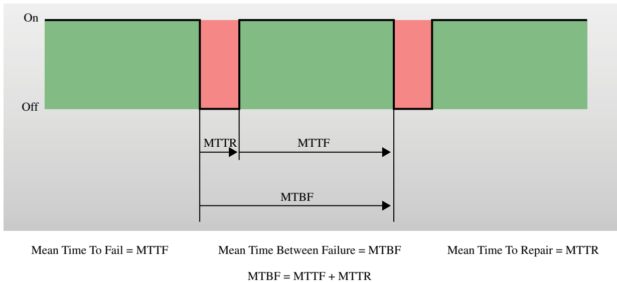
FIGURE 11.12 Availability time diagram.
