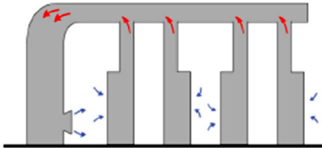
FIGURE 24.3 Fully ducted return—flooded supply. Courtesy of Schneider Electric.
