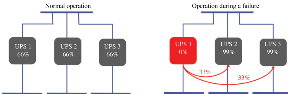
FIGURE 11.6 N+1 normal operation and failure scenarios.
