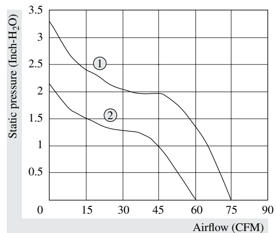
FIGURE 26.7 Fan curves 60 mm × 60 mm.
