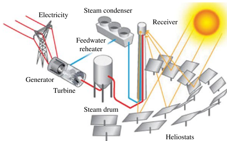
FIGURE 30.1 Solar power tower energy plant. Plant illustration from Energy Efficiency and Renewable Energy (EERE), U.S. Department of Energy.
