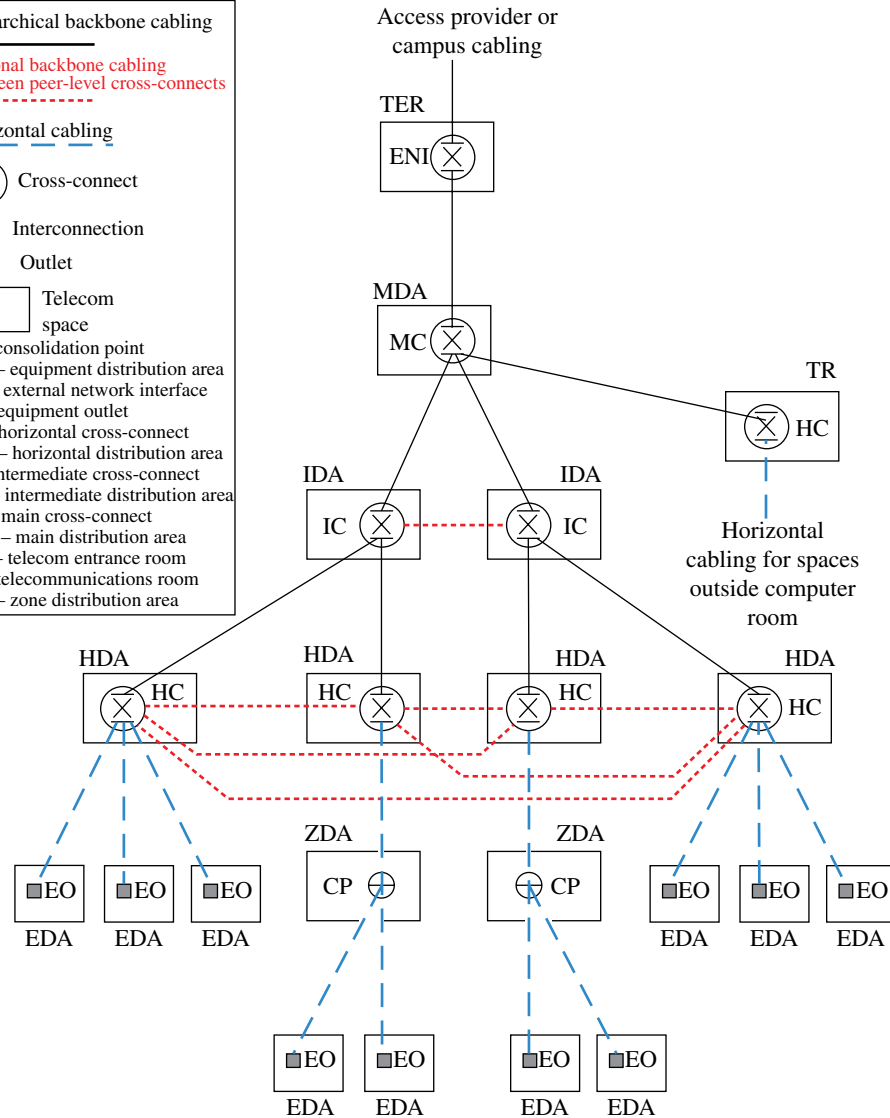
FIGURE 14.7 Hierarchical star topology.
