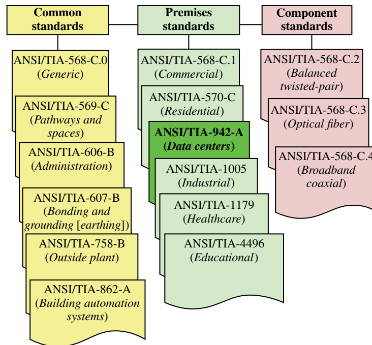
FIGURE 14.3 Organization of TIA telecommunications cabling standards.
