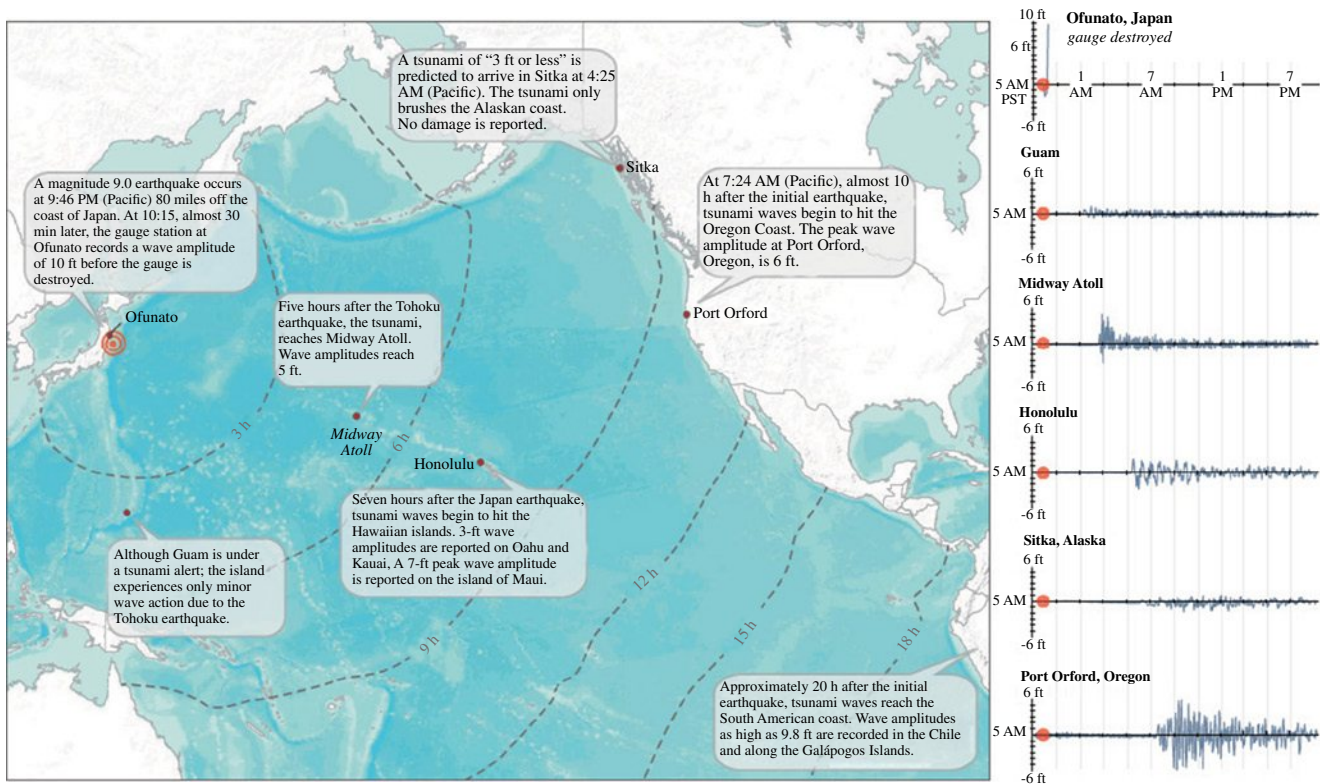
FIGURE 36.2 Progression of the Tohoku tsunami across the Pacific Ocean with tide gauge water level measurements showing deviation from predicted tide levels. From http://tidesandcurrents.noaa.gov/
