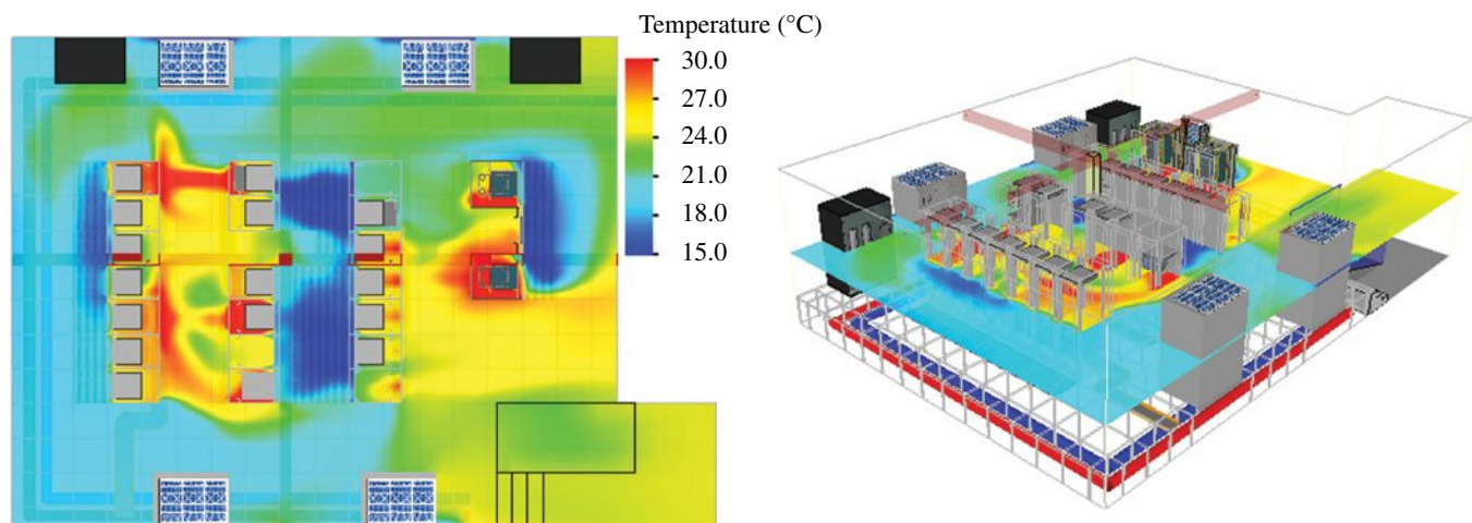
FIGURE 17.6 Result plane of temperature and halfway cabinet. Courtesy of Future Facilities. Please visit companion website to access the color version of this figure.
