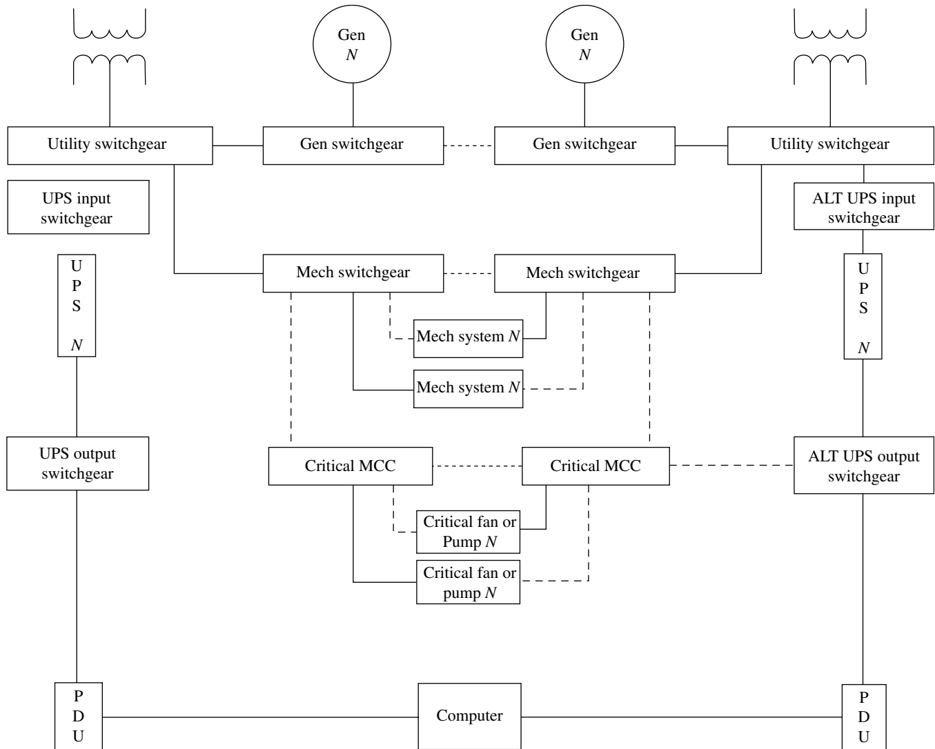
FIGURE 35.8 Uptime Institute Tier 4 indicative electrical system design.
