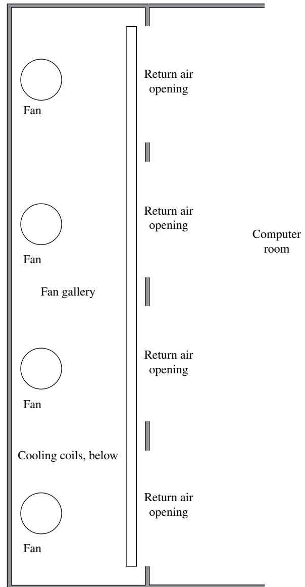
FIGURE 9.8 Example of Fan Gallery (plan view). Courtesy of Isaak Technologies.
