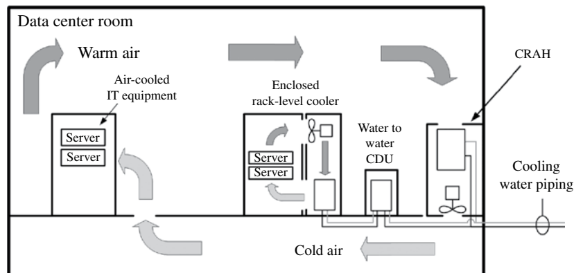
FIGURE 26.3 Side view: Enclosed rack-level cooler installation.
