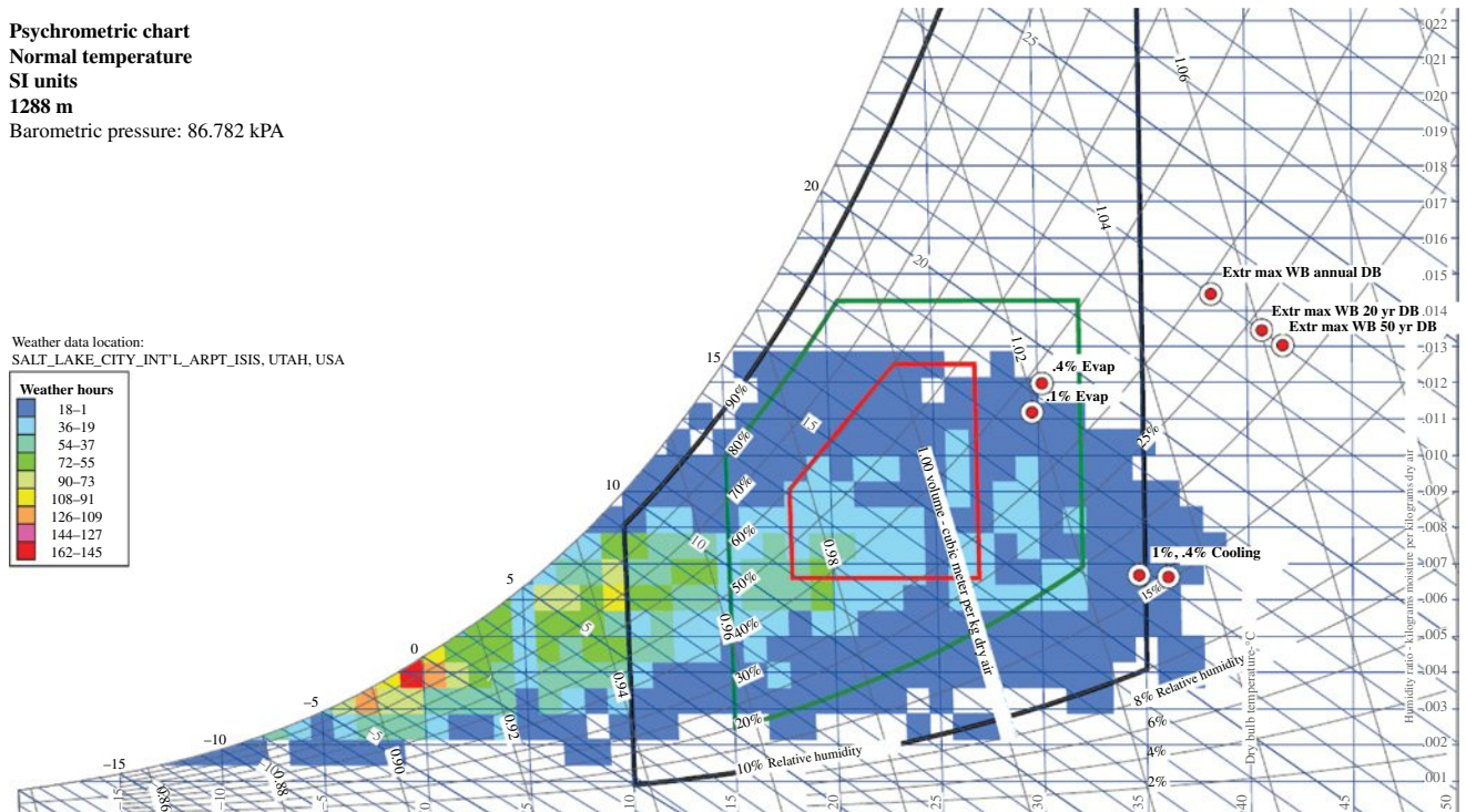
FIGURE 4.11 Cooling technology module choices must take into account extremes as well as typical. Courtesy of Hewlett-Packard Company.
