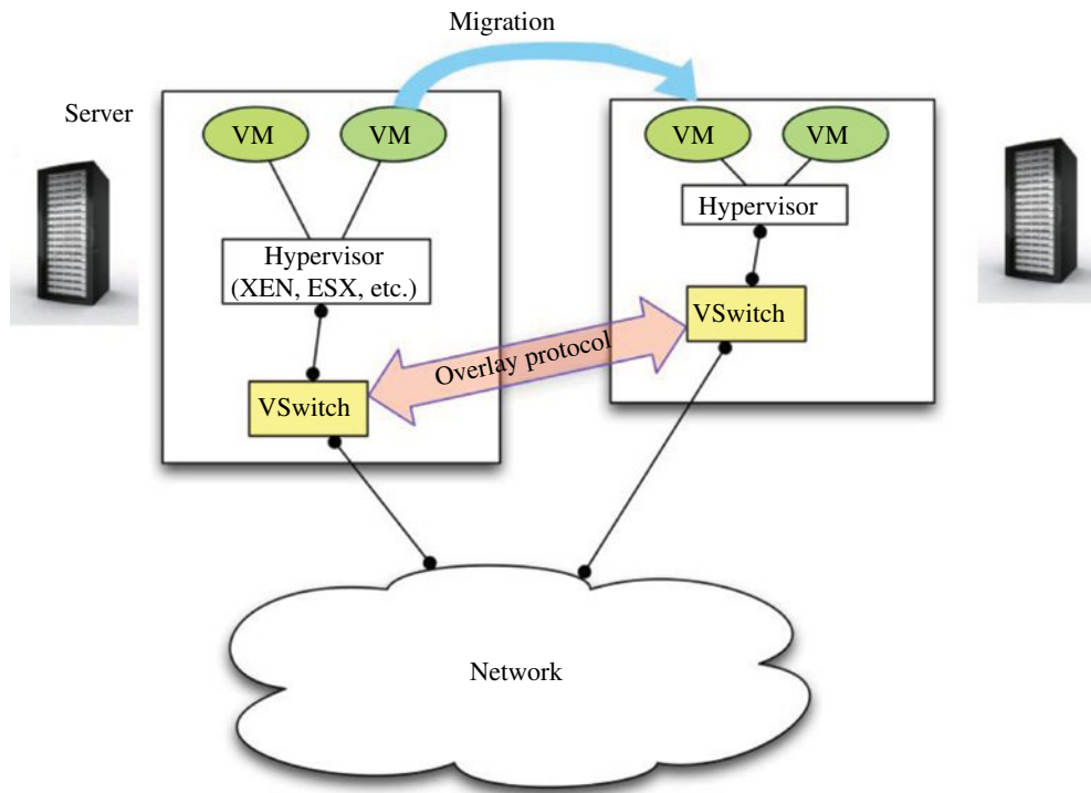
FIGURE 20.1 Migration of a VM in a data center.
