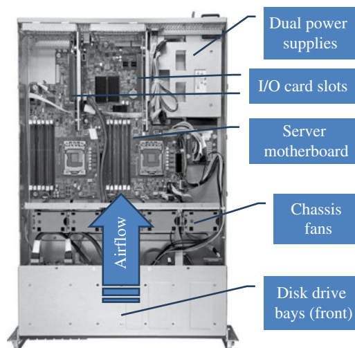
FIGURE 21.5 Typical 2U, Dual-Processor (DP) Rack Server seen from the top with the cover removed. Airflow is front to back through the rack. Note that the two microprocessors and their heat sinks are not installed, neither is the second PSU. Courtesy of Intel Corporation.
