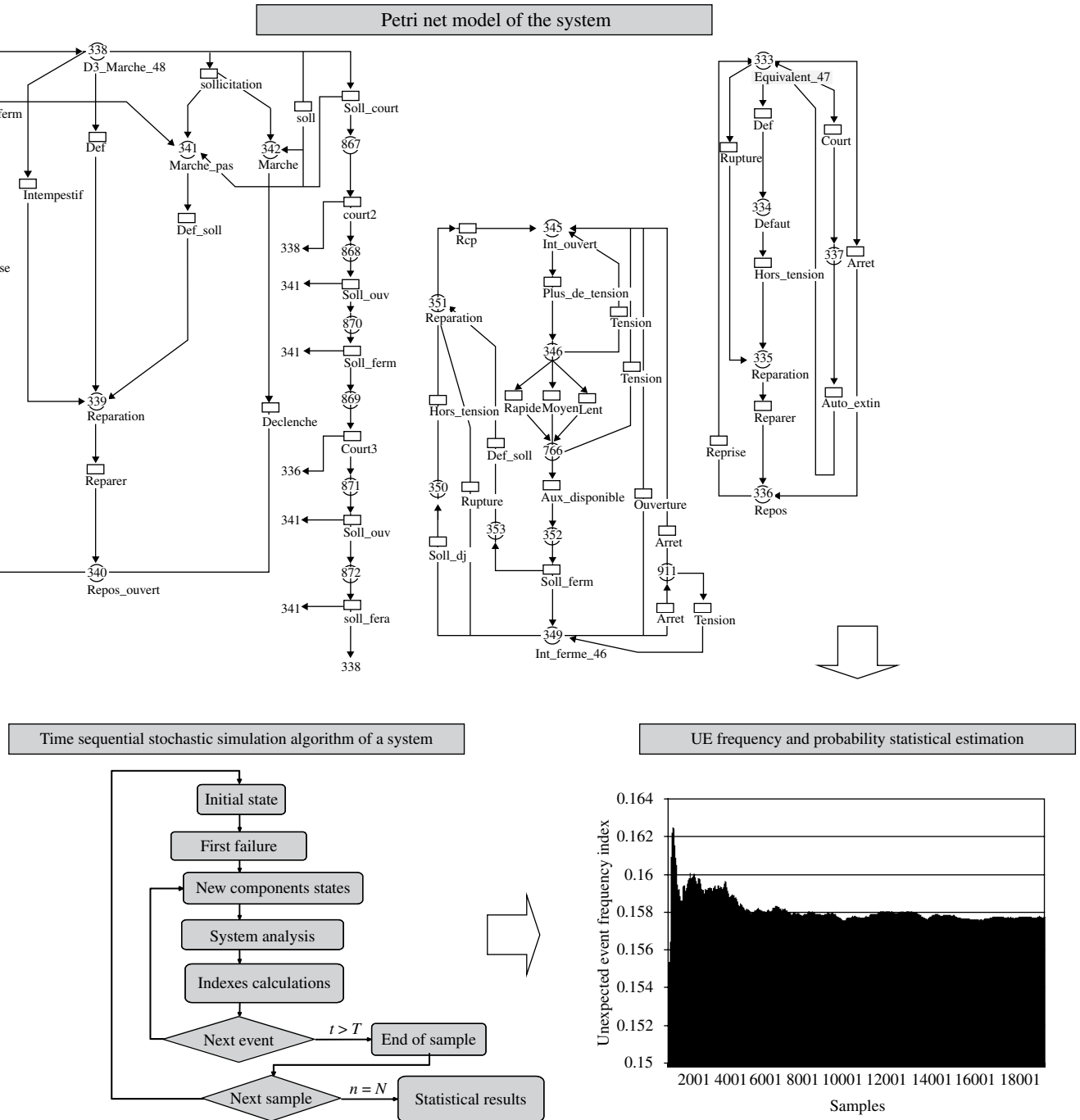
FIGURE 15.24 Time sequential stochastic simulation algorithm of a system.
