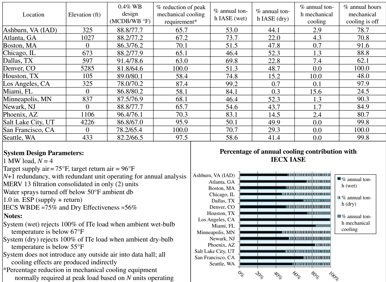
FIGURE 25.13 Analysis summary for modular data center cooling solution using IECX.
