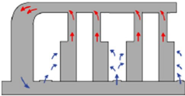
FIGURE 24.4 Fully ducted return—locally ducted supply (Left, Raised floor; Right, Overhead). Courtesy of Schneider Electric.
