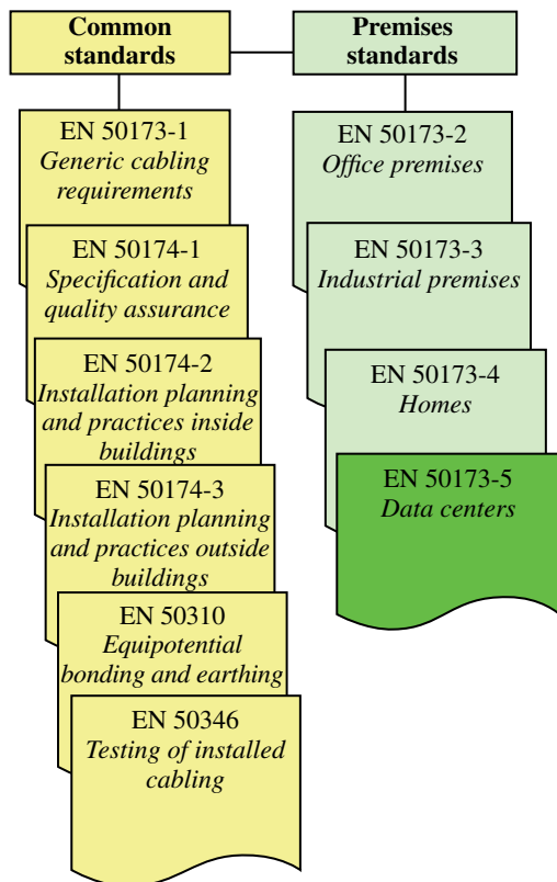
FIGURE 14.4 Organization of CENELEC telecommunications cabling standards.
